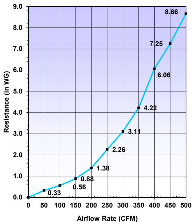
Air Flow vs Resistance
