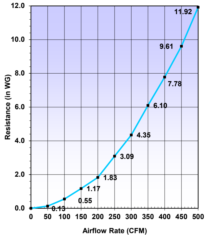
Air Flow vs Resistance
